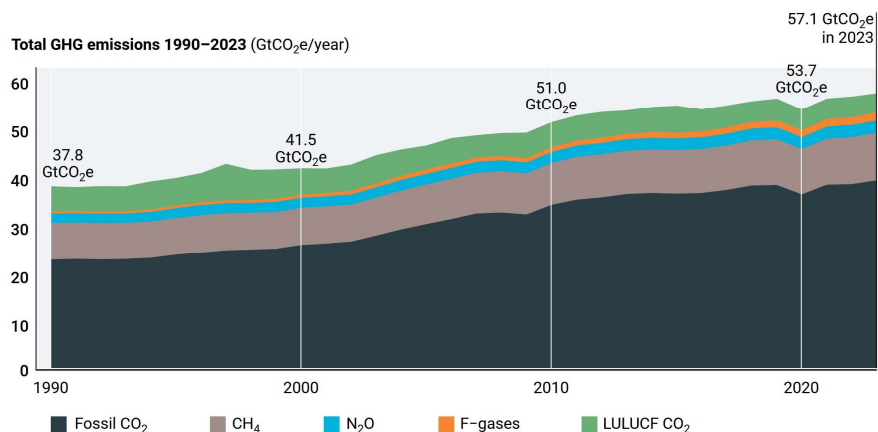
Figure 2.1 Total net anthropogenic GHG emissions, 1990–2023
