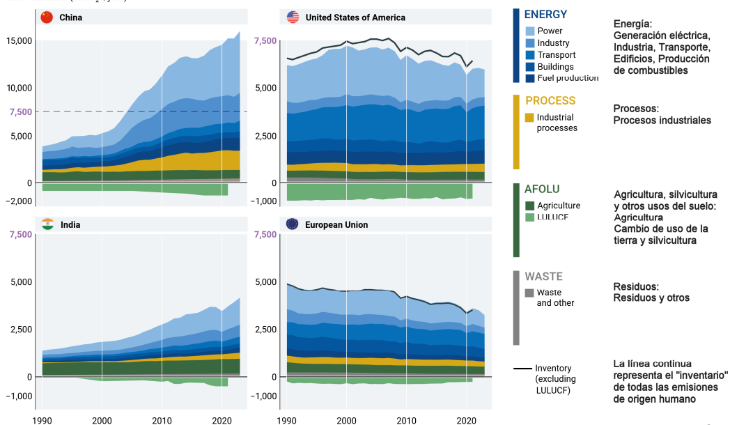
GHG emissions (MtCO 2 e/year)
